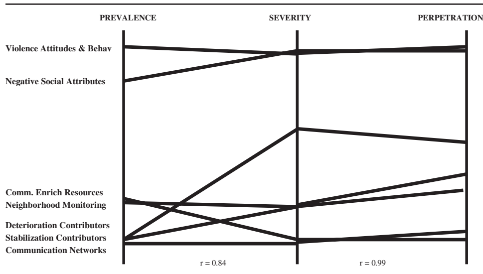
FIGURE 8: Pattern-Matching Results
